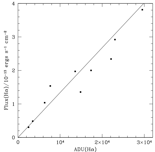
FIG. 5.—ADU vs. flux relation for the calibration H II regions listed in Table 3. Flux is given in units of 10^{-13} \text{ ergs s}^{-1} \text{ cm}^{-2} . The solid line represents the relation given by equation (3).
