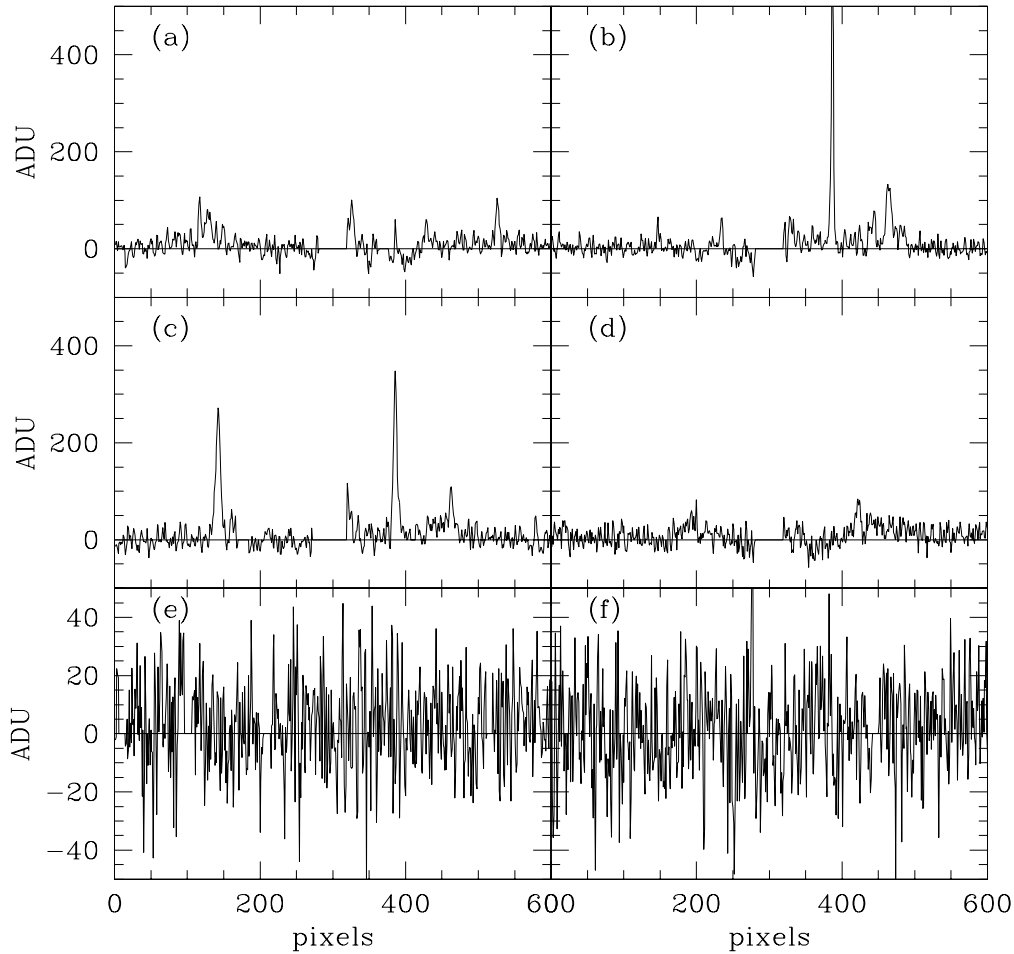
FIG. 4.—Six slices through Fig. 3 that are each 1 pixel wide and 600 pixels long, shown as dotted lines in Fig. 3. Slices (a), (b), (c), and (d) each go through the center of M81 and a few H II regions, with the galaxy center located at pixel 300 in each slice. Slice (a) is along a diagonal that goes from bottom left to top right, while slice (b) is a diagonal that goes from top left to bottom right. Slices (c) and (d) are cuts along the X and Y directions, respectively. In slices (a)–(d), the galaxy center H \alpha goes off scale. Slices (e) and (f) are cuts along the Y direction through the left and right regions in Fig. 3 where there are no H II regions.
